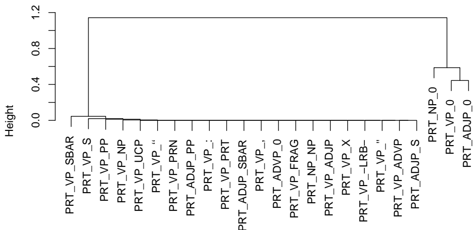
Figure 3: Dendrogram for particle (PRT) contextualized with mother-right-sister
